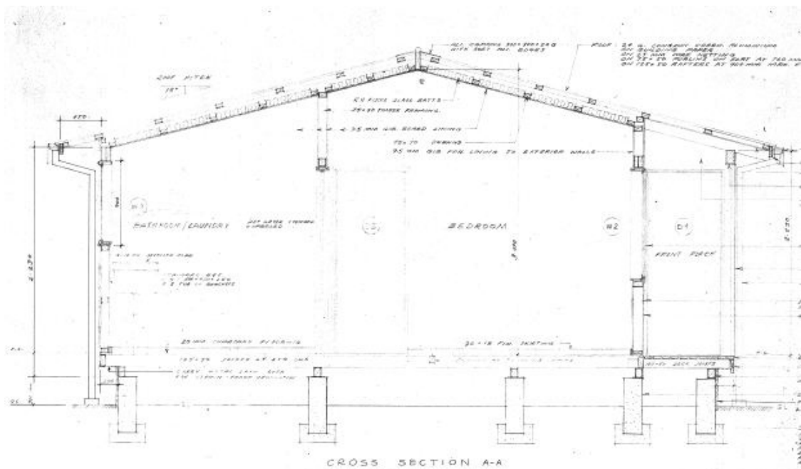
Figure 5: Cross section of Forfar Courts s.
