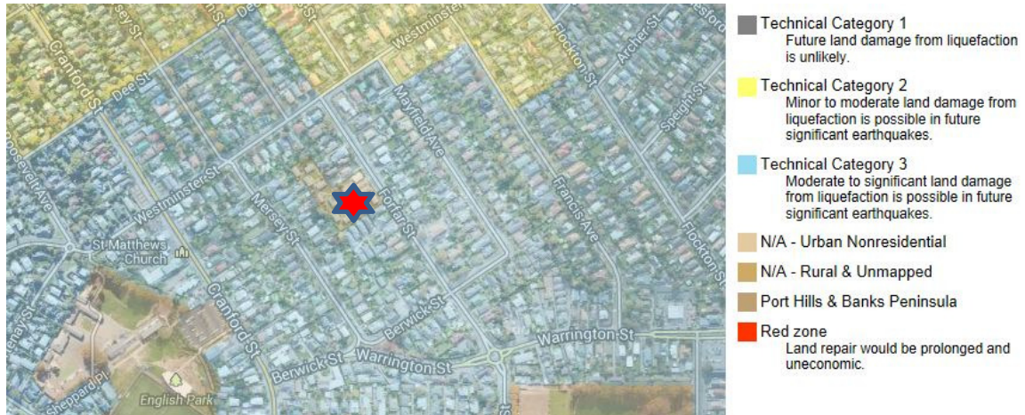
Figure 12: CERA Technical Categories map (loc. starred).
