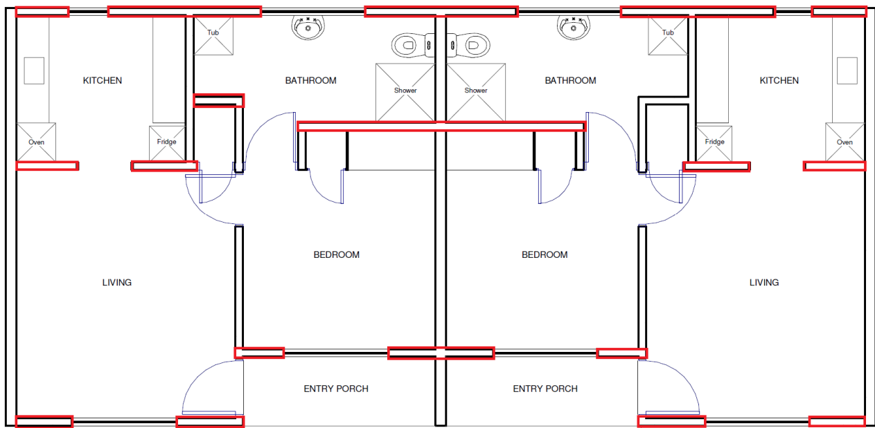
Figure 8: Walls used for bracing in the longitudinal direction (Residential Units).
