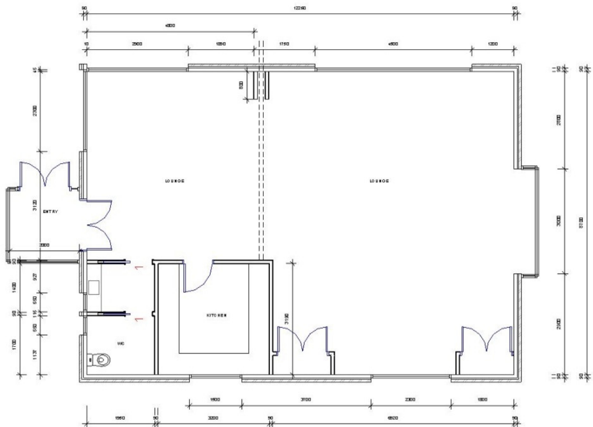
Figure 6: Floor plan of Residents Lounge.
