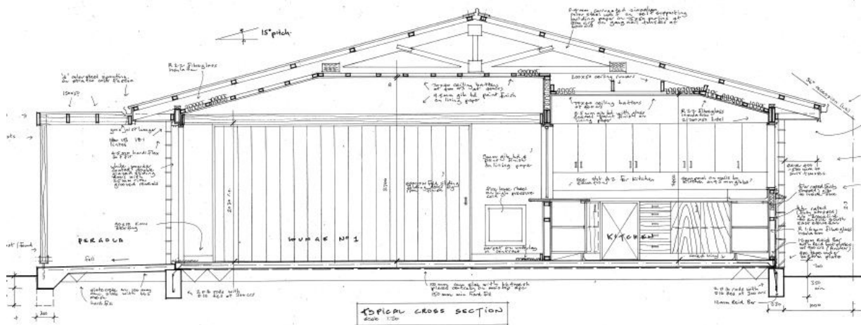
Figure 7: Cross section of Residents Lounge.
