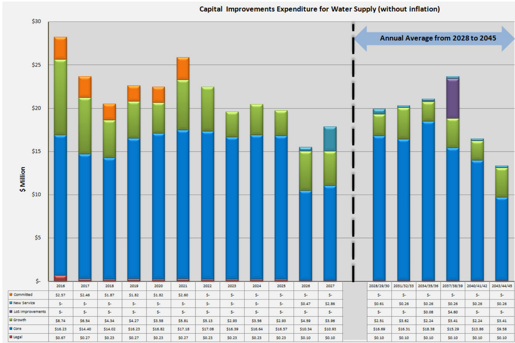
Figure 7-6: Capital Expenditure – Water Supply (without inflation)
