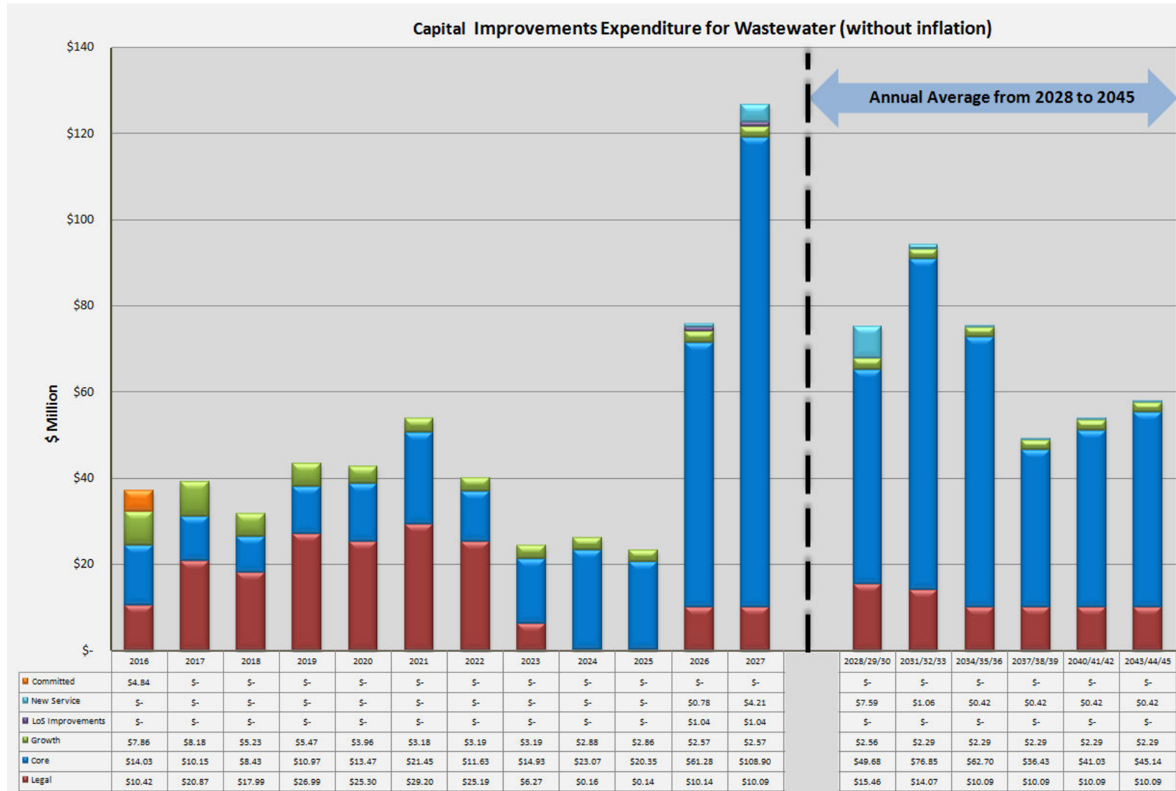
Figure 7-8: Capital Expenditure – Wastewater (without inflation)
