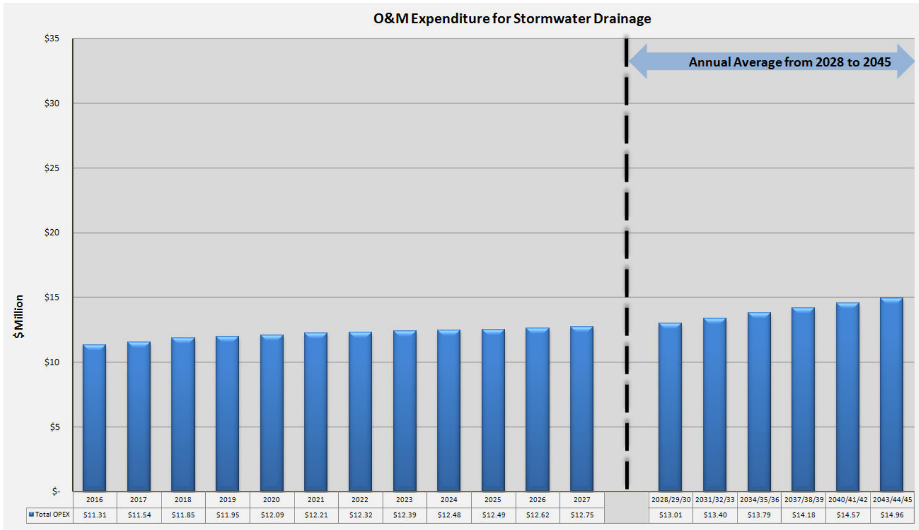
Figure 7-9: Operations and Maintenance Expenditure – Stormwater (without inflation)
