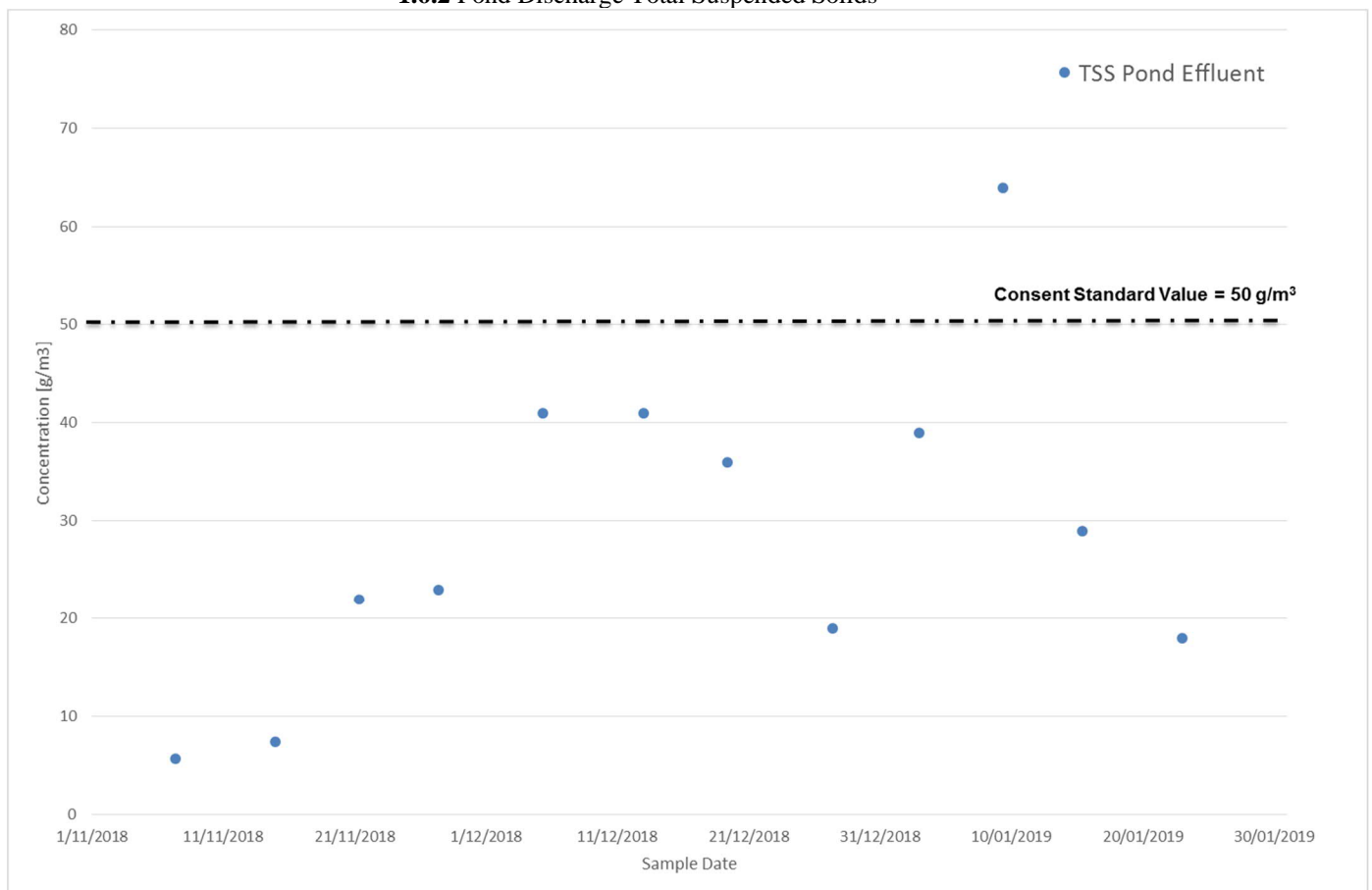
1.6.2 Pond Discharge Total Suspended Solids
