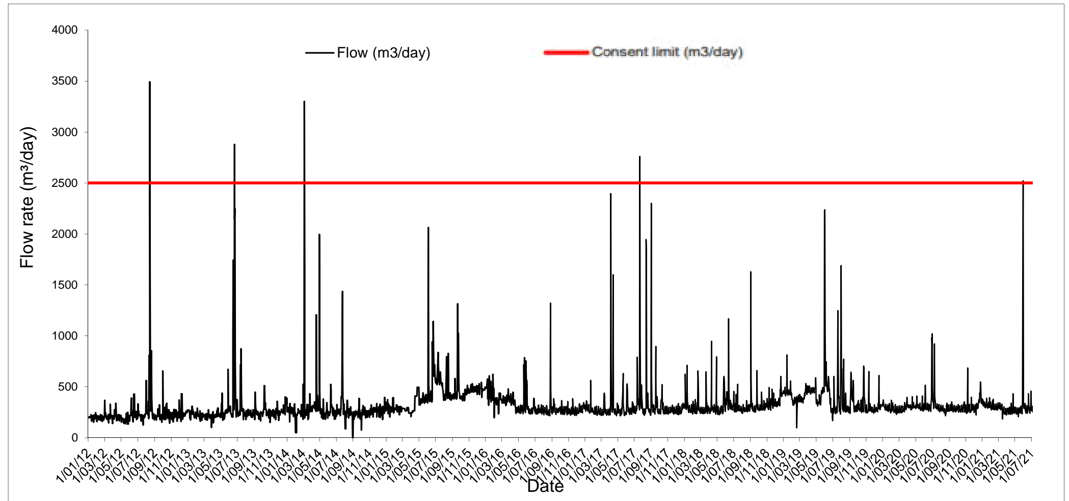
Figure 1: The daily quantity of treated water from 2012 to present at Diamond Harbour wastewater treatment plant.
