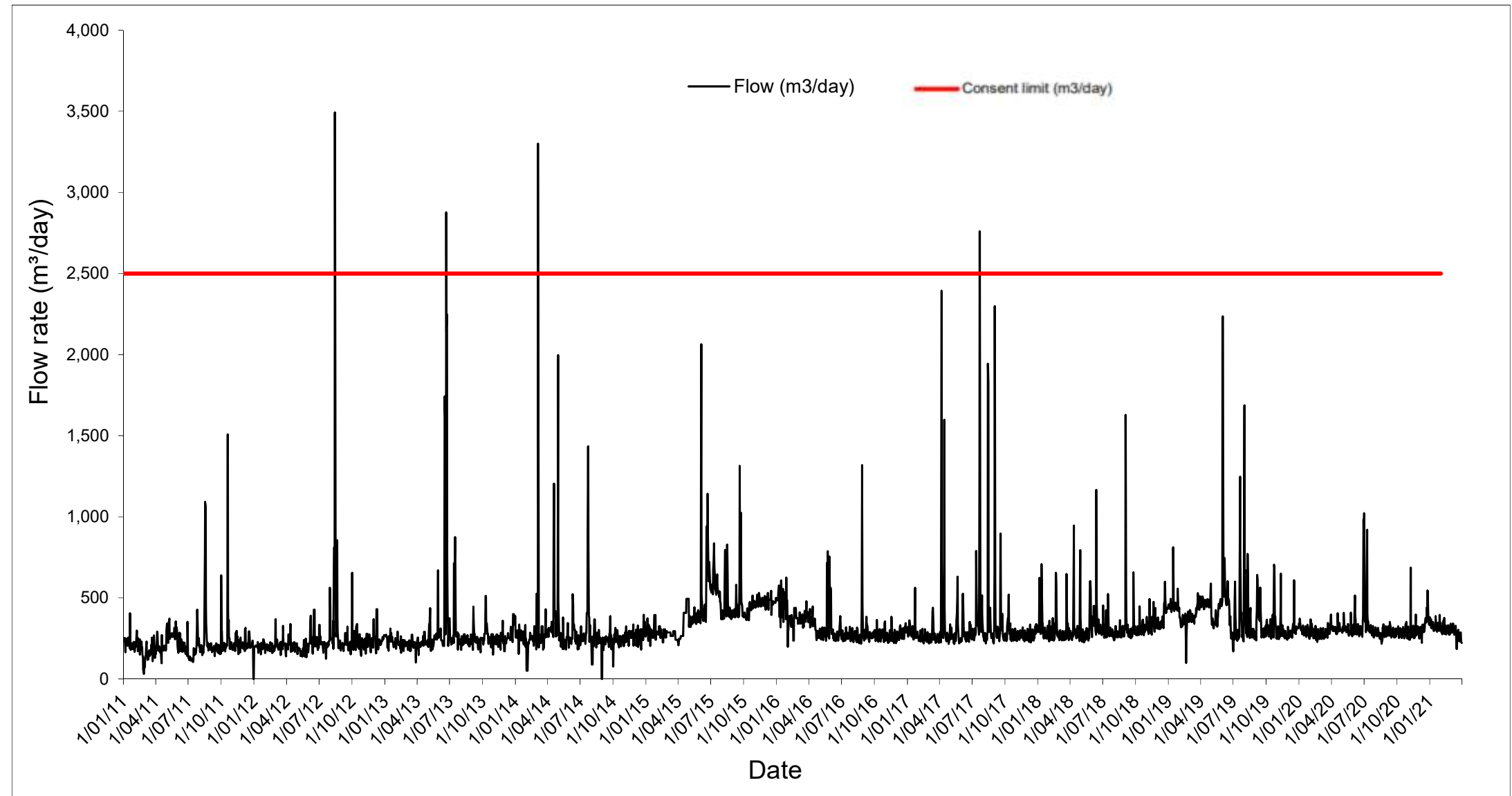
Figure 1: The daily quantity of treated water from 2012 to present at Diamond Harbour wastewater treatment plant.
