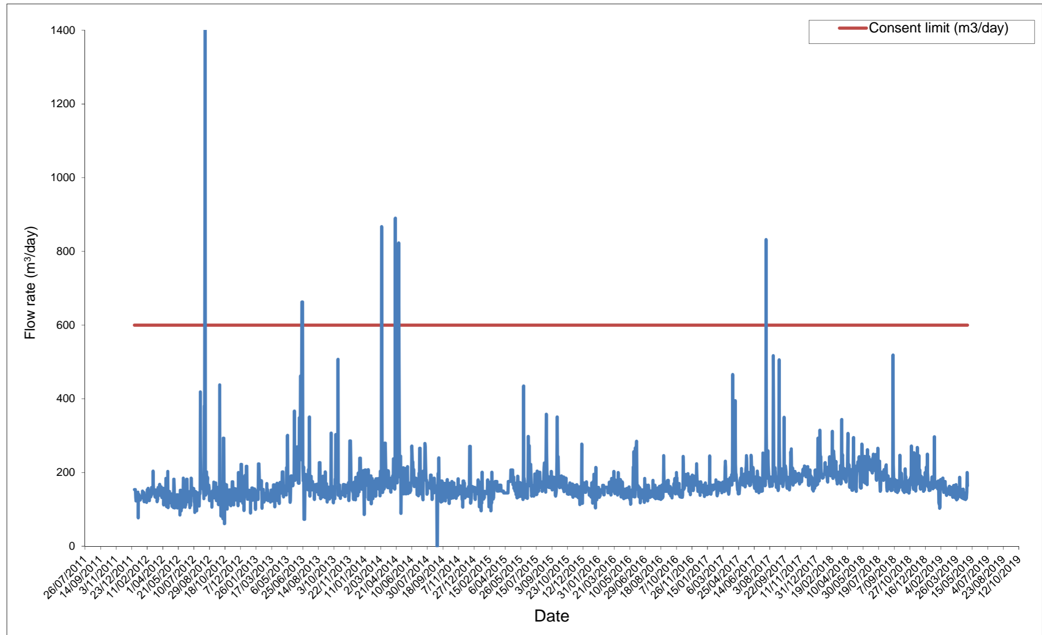
Figure 1: The daily quantity of treated water from the Governors Bay wastewater treatment plant 2012 to present
