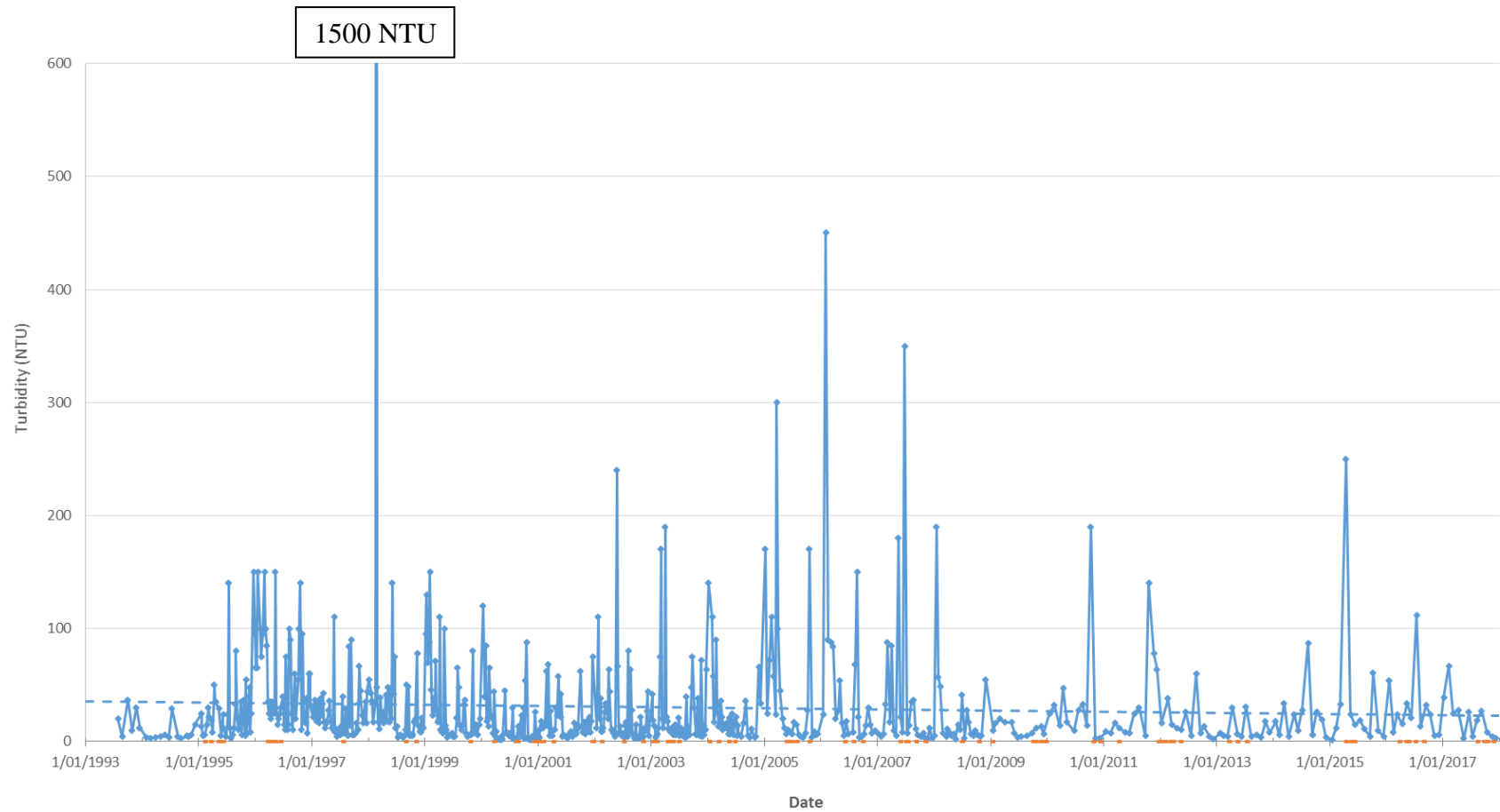
Figure 5. Turbidity of water at Wairewa/Lake Forsyth at the water level recording site for the entire dataset (July 1993 - December 2017). The dashed line is a linear trendline. One data point is significantly higher than the other data points and is therefore off the scale of the graph – the text box details the concentration of this sample.
