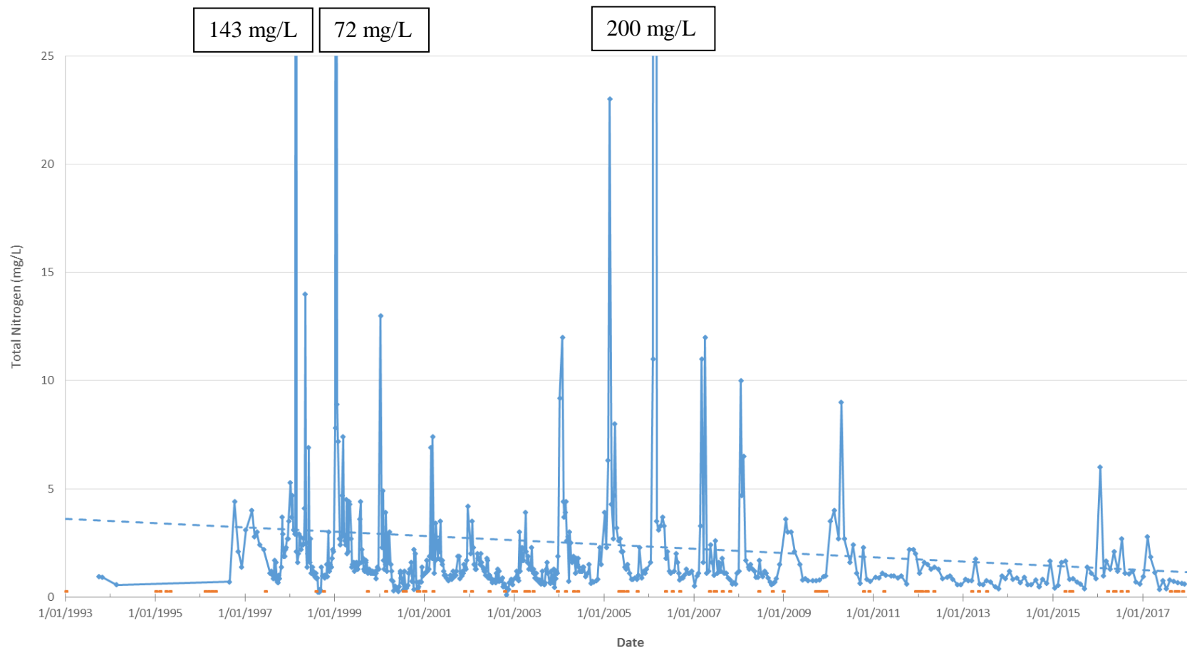
Figure 6. Total Nitrogen at Wairewa/Lake Forsyth at the ECan Water Level Recorder site for the entire dataset (July 1993 – December 2017). The dashed line is a linear trendline. Three data points are significantly higher than the other data points and are therefore off the scale of the graph – the text boxes detail their concentrations.
