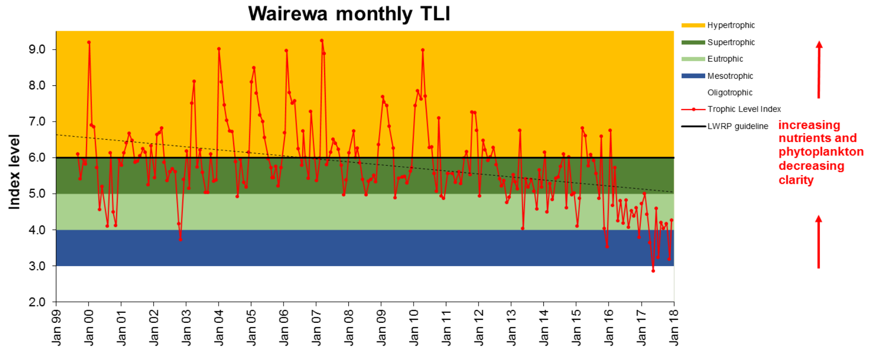
Figure 8a. Trophic Level Index (TLI) at Wairewa/Lake Forsyth at the ECan Water Level Recorder site for the entire dataset (September 1999 – December 2017). The dashed line is a linear trendline. Solid black line = Land and Water Regional Plan (LWRP) guideline for coastal lakes (6). Graph modified from Environment Canterbury versions.
