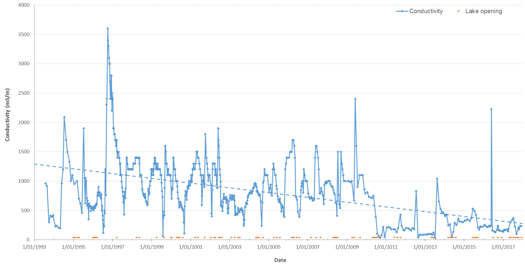
Figure 2. Conductivity of water at Wairewa/Lake Forsyth at the ECan Water Level Recorder site for the entire dataset (July 1993 - December 2017). The dashed line is a linear trendline.
