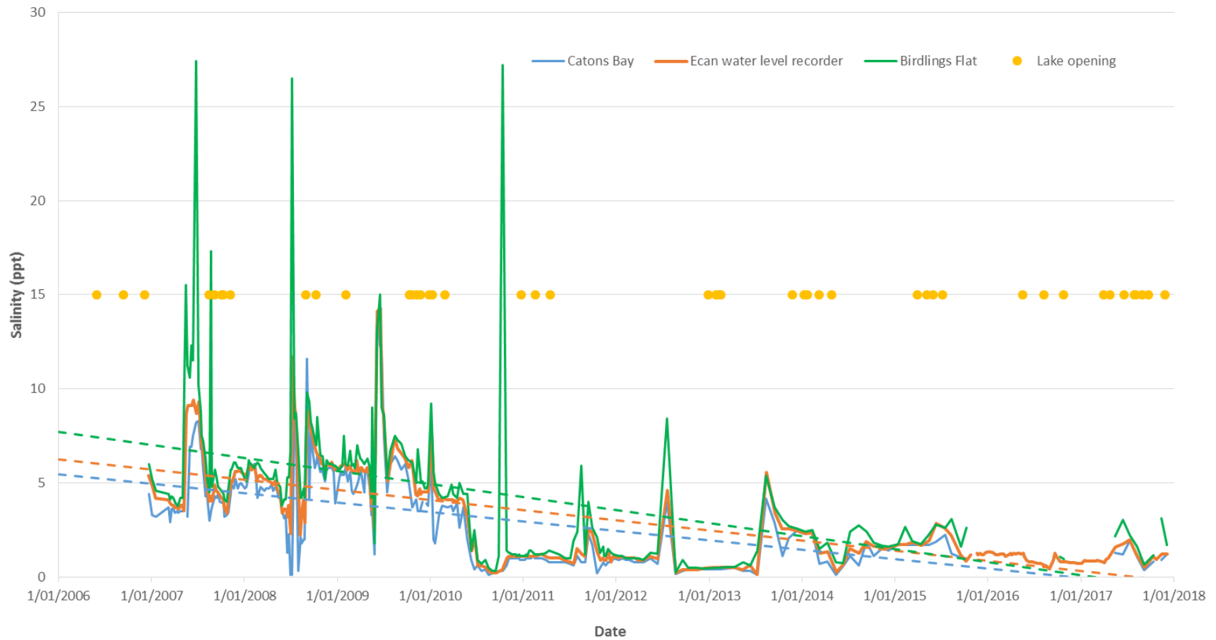
Figure 3. Salinity of water at Wairewa/Lake Forsyth at three sites (ECan Water Level Recorder, Catons Bay and Birdlings Flat) from the entire dataset (December 2006 - December 2017). The dashed lines are linear trendlines.
