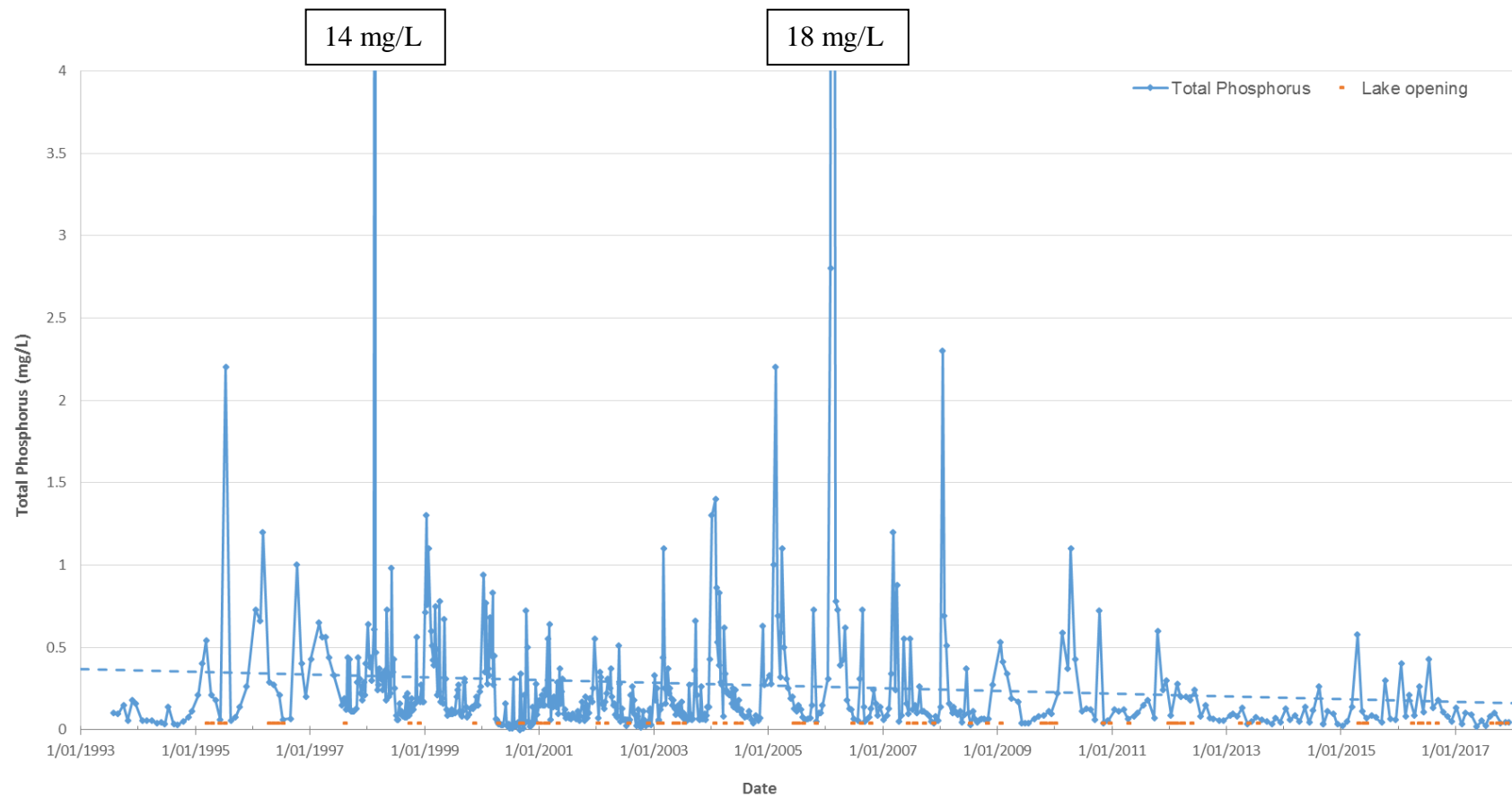
Figure 7. Total phosphorus at Wairewa/Lake Forsyth at the ECan Water Level Recorder site for the entire dataset (July 1993 – December 2017). The dashed line is a linear trendline. Two data points are significantly higher than the other data points and are therefore off the scale of the graph – the text boxes detail their concentrations.
