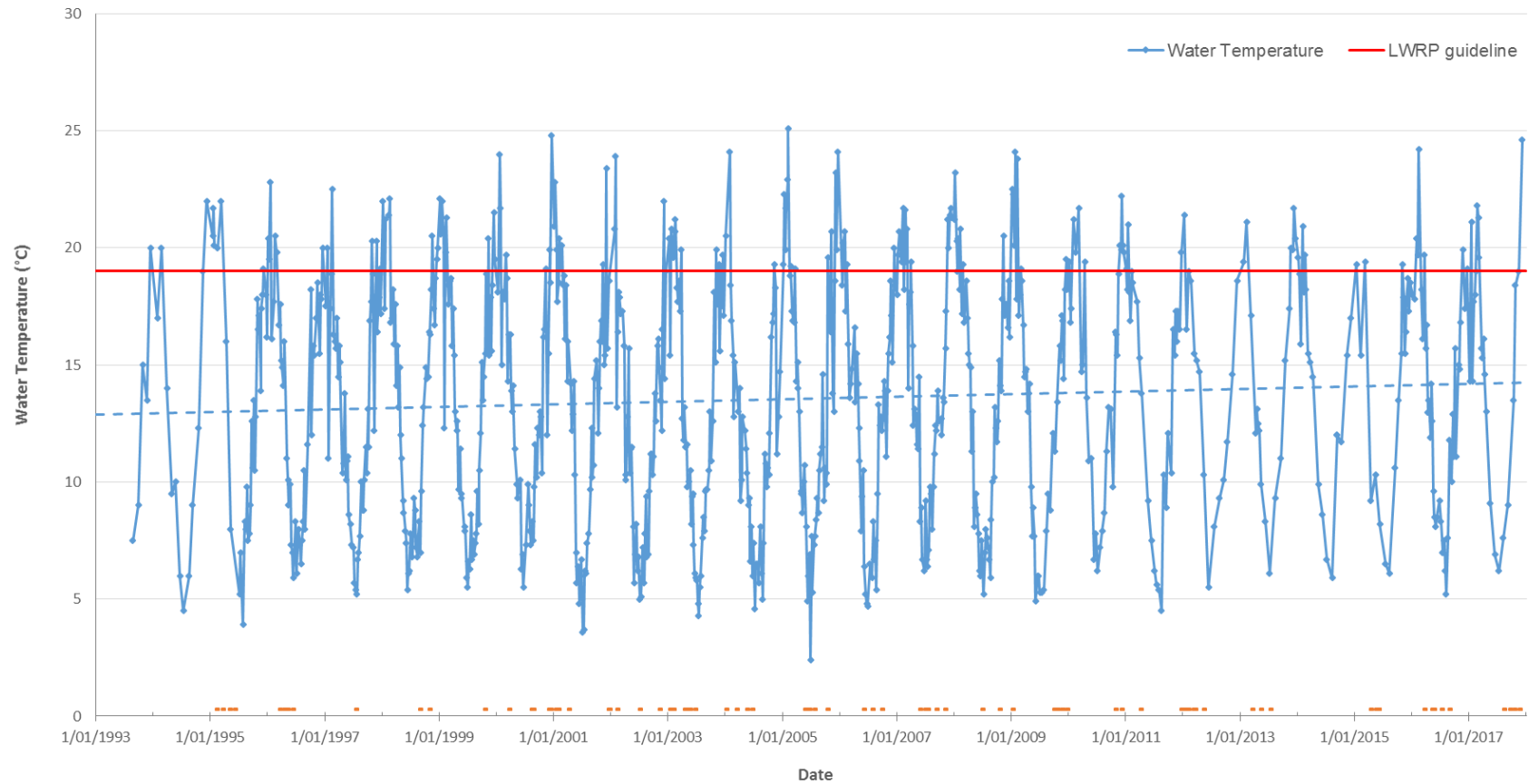
Figure 4. Water Temperature at Wairewa/Lake Forsyth at the ECan Water Level Recorder site for the entire dataset (August 1993 - December 2017). The dashed line is a linear trendline. Red line = Land and Water Regional Plan (LWRP) guideline for coastal lakes (19°C).
