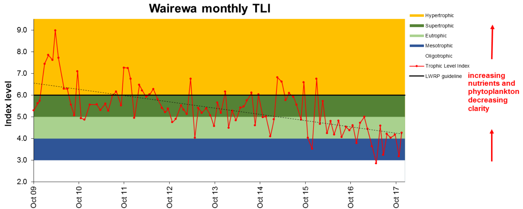
Figure 8c. Trophic Level Index (TLI) at Wairewa/Lake Forsyth at the ECan Water Level Recorder site after the construction of the canal opening (October 2009– December 2017). The dashed line is a linear trendline. Solid black line = Land and Water Regional Plan (LWRP) guideline for coastal lakes (6). Graph modified from Environment Canterbury versions.
