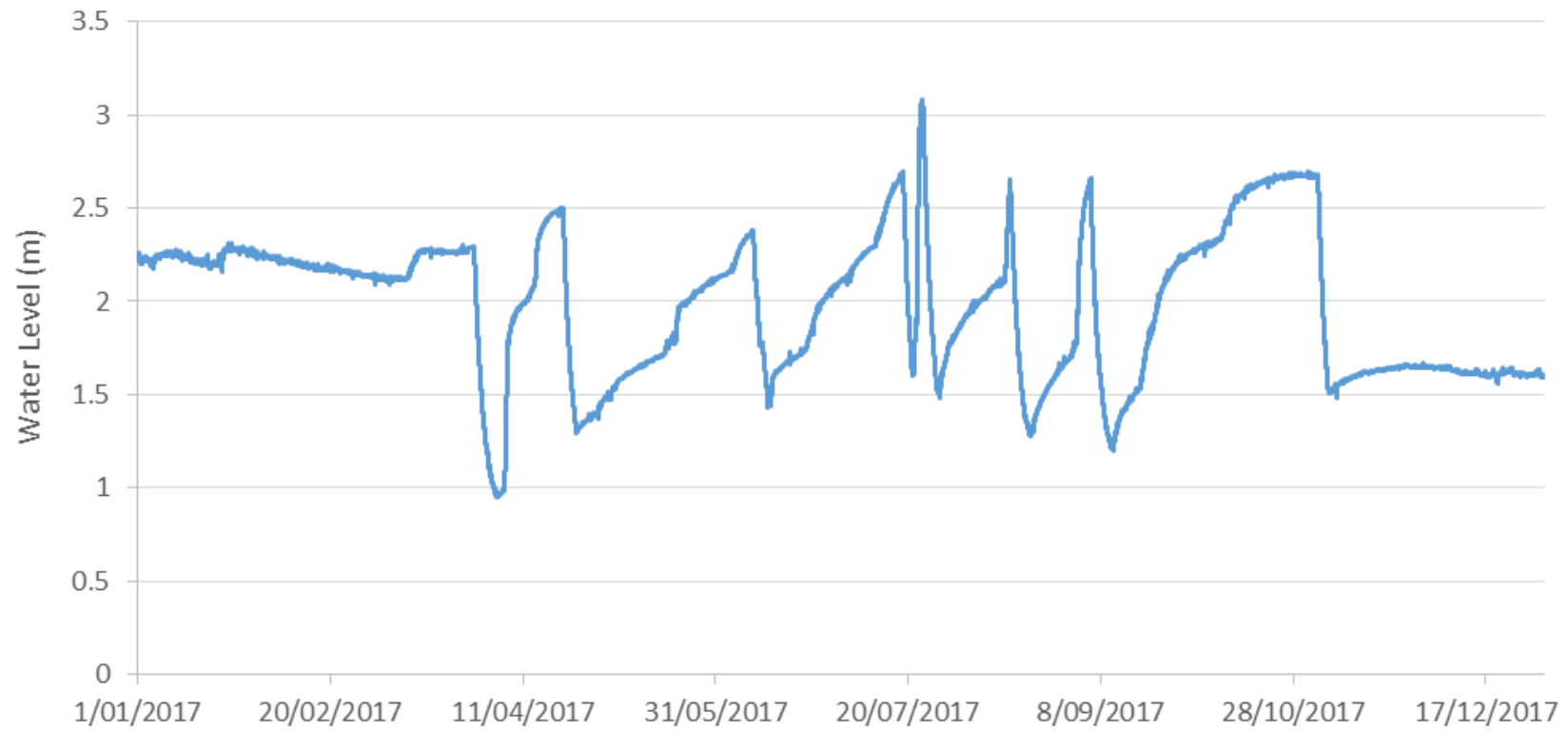
Figure 13. Water level in Lake Forsyth/Te Wairewa. Sharp drops in water level indicate when the lake was opened.
