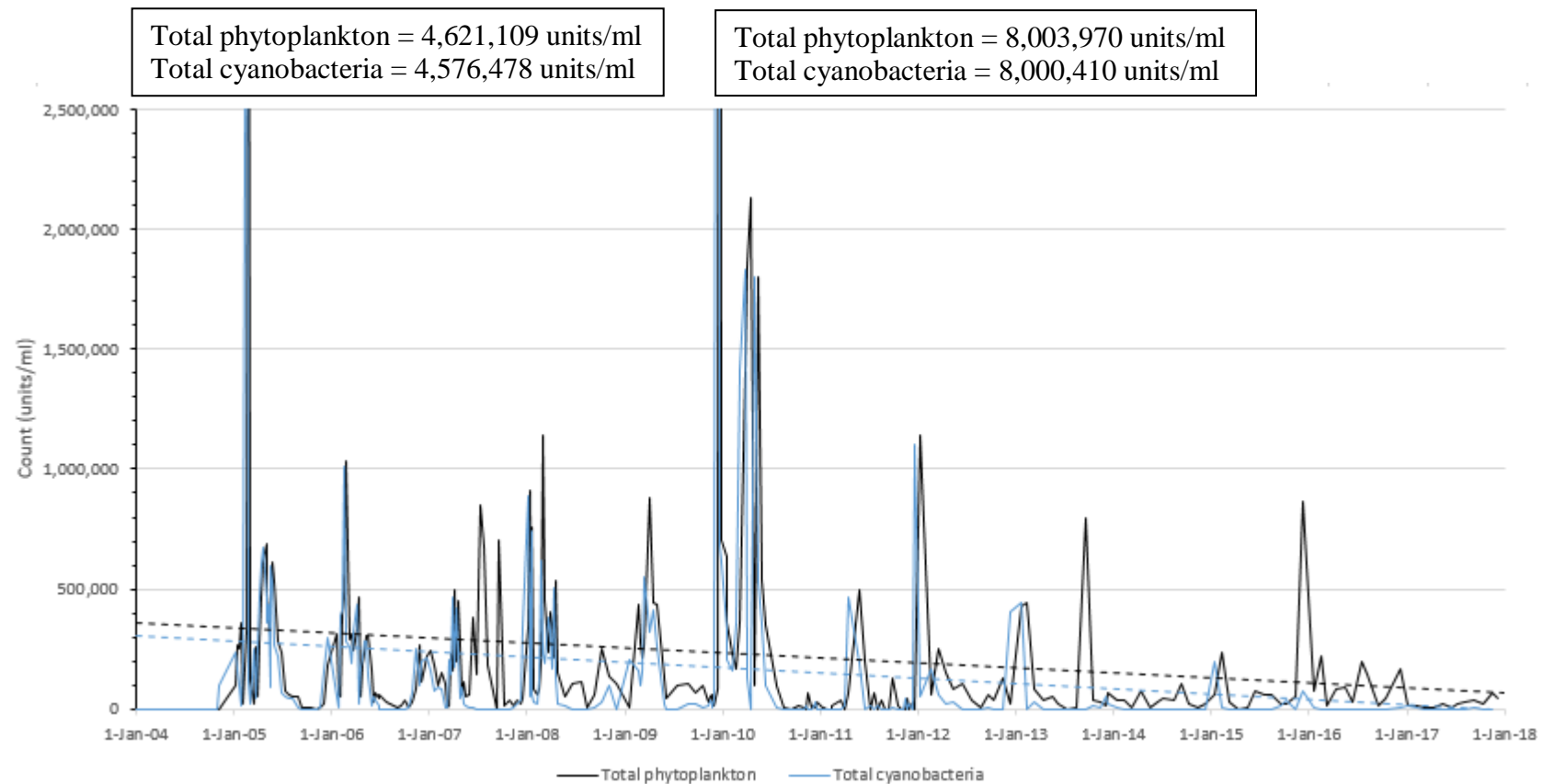
Figure 9. Total phytoplankton and cyanobacteria (a subset of phytoplankton) counts at Wairewa/Lake Forsyth at the ECan Water Level Recorder site from September 2004 to December 2017. The dashed lines are linear trendlines. Two data points are significantly higher than the other data points and are therefore off the scale of the graph – the text boxes detail their concentrations.
