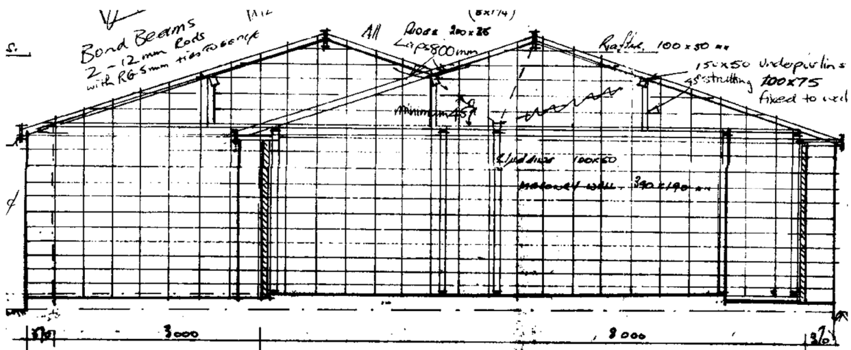
Figure 5: Cross section (fire wall) of Thames Courts.
