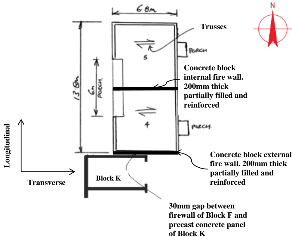
Figure 2 Plan sketch show key structural elements
