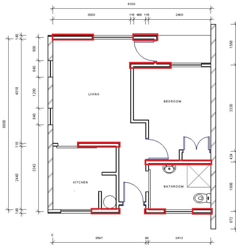
Figure 6: Walls used for bracing in the longitudinal direction.
