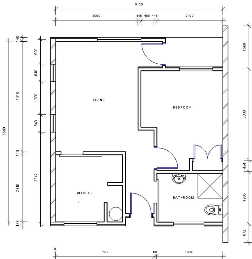
Figure 4: Typical partial floor plan of residential unit blocks.
