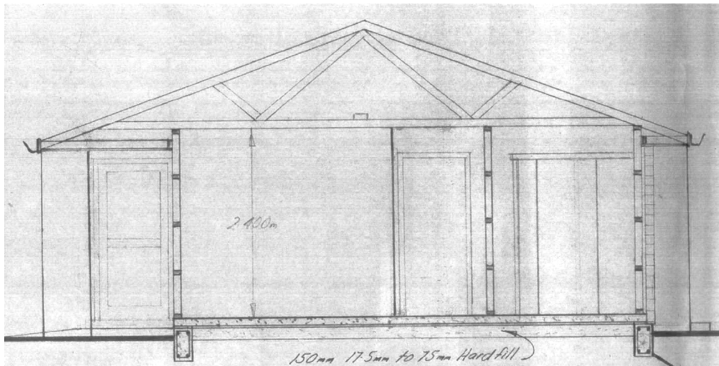
Figure 5: Cross section of Gayhurst Road Housing Complex.
