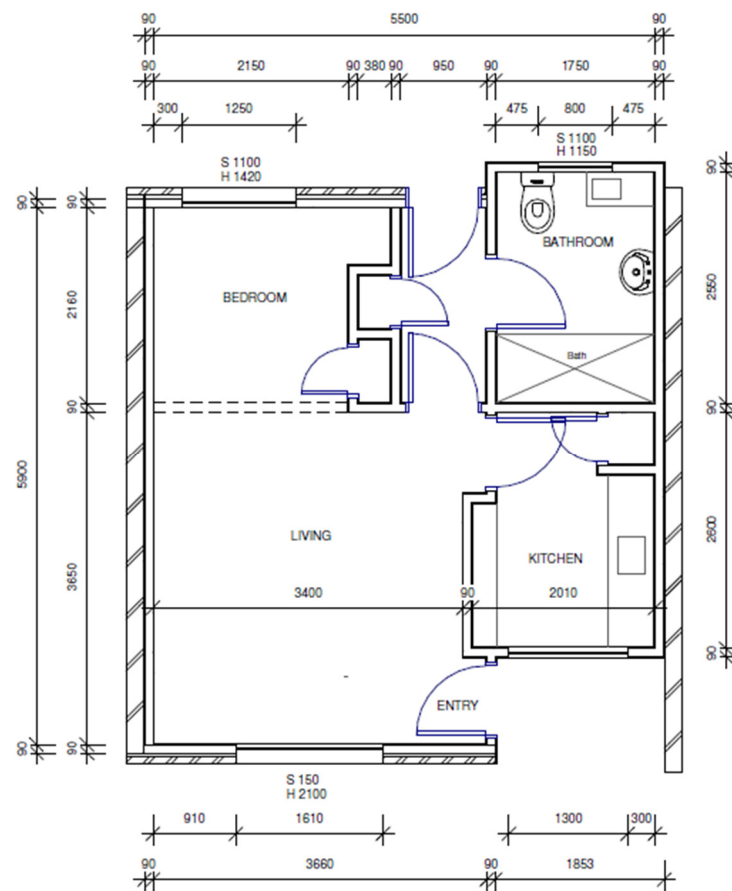
Figure 4: Partial floor plan of residential unit blocks.
