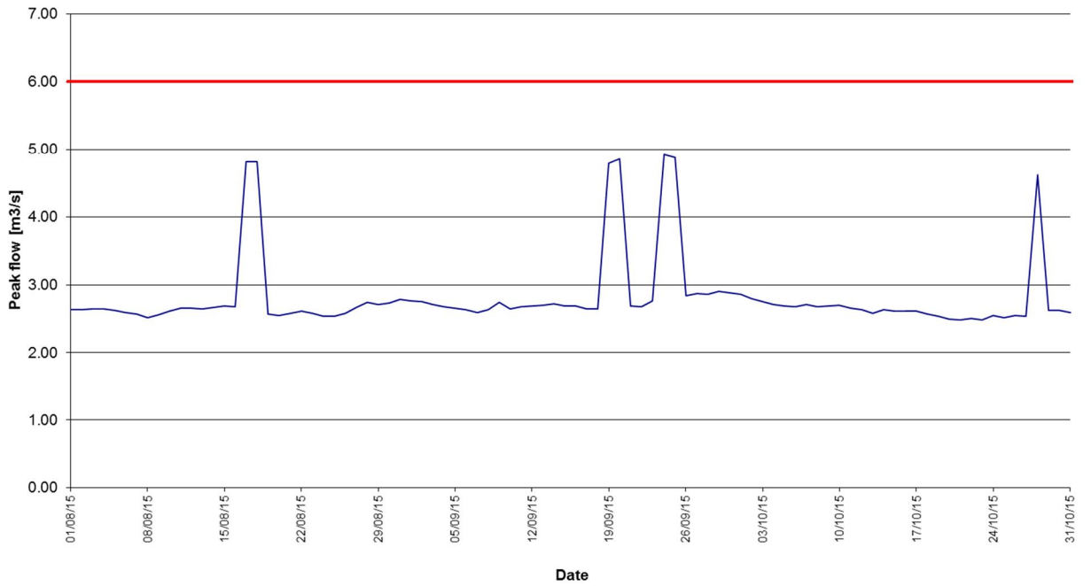
Figure 1.2.2 - Daily Peak Outfall Flows
