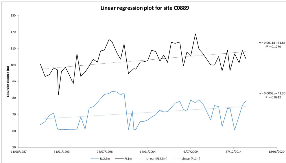
Figure B10 Beach profile surveys (top panel) and linear regression plots for RL 2.5 m and RL 1 m contours (lower panel) for profile C0889
