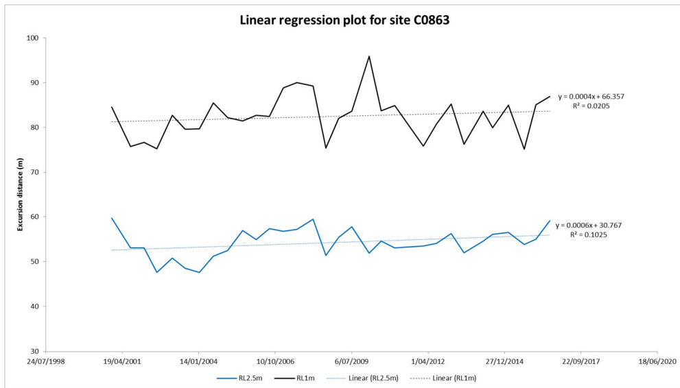
Figure B11 Beach profile surveys (top panel) and linear regression plots for RL 2.5 m and RL 1 m contours (lower panel) for profile C0863
