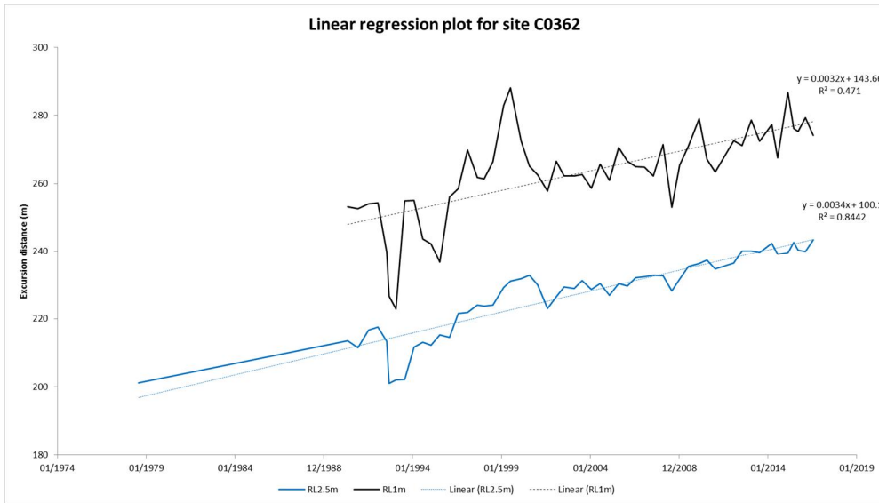
Figure B26 Beach profile surveys (top panel) and linear regression plots for RL 2.5 m and RL 1 m contours (lower panel) for profile C0362
