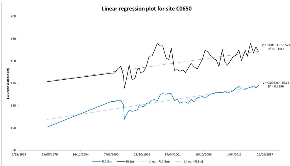
Figure B19 Beach profile surveys (top panel) and linear regression plots for RL 2.5 m and RL 1 m contours (lower panel) for profile C0650
