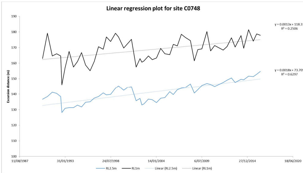
Figure B17 Beach profile surveys (top panel) and linear regression plots for RL 2.5 m and RL 1 m contours (lower panel) for profile C0748
