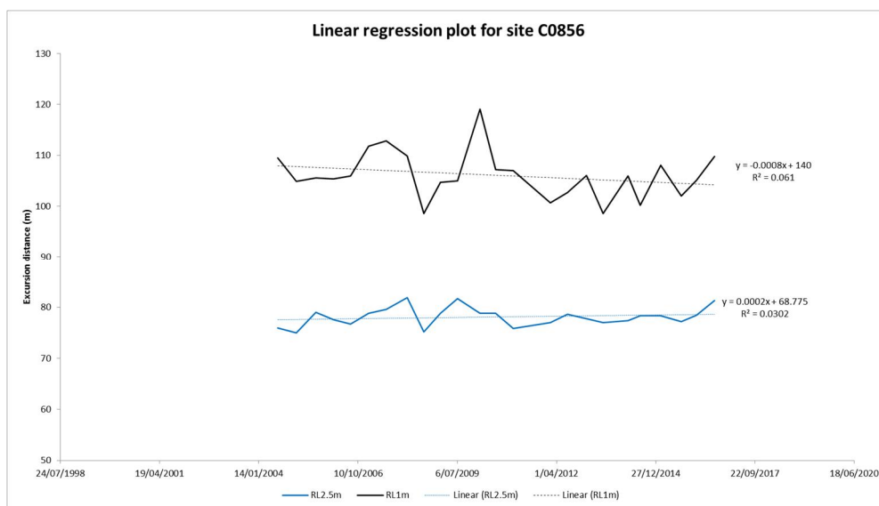
Figure B12 Beach profile surveys (top panel) and linear regression plots for RL 2.5 m and RL 1 m contours (lower panel) for profile C0856
