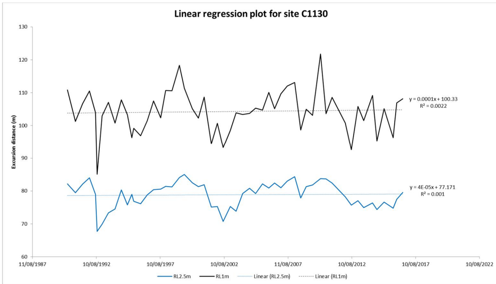
Figure B1 Beach profile surveys (top panel) and linear regression plots for RL 2.5 m and RL 1 m contours (lower panel) for profile C1130
