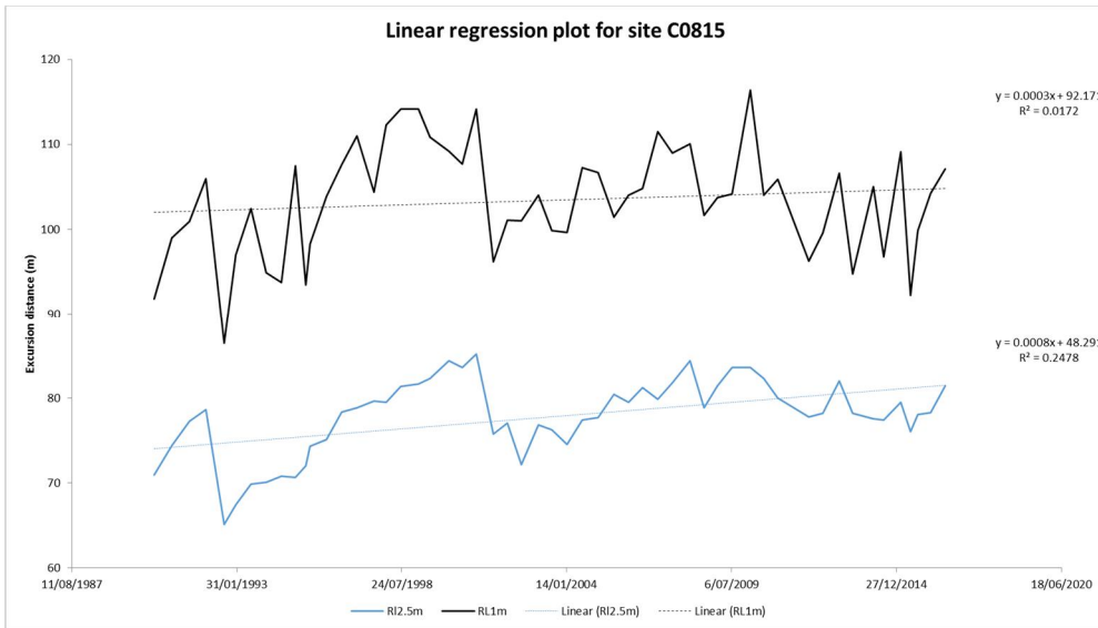
Figure B15 Beach profile surveys (top panel) and linear regression plots for RL 2.5 m and RL 1 m contours (lower panel) for profile C0815
