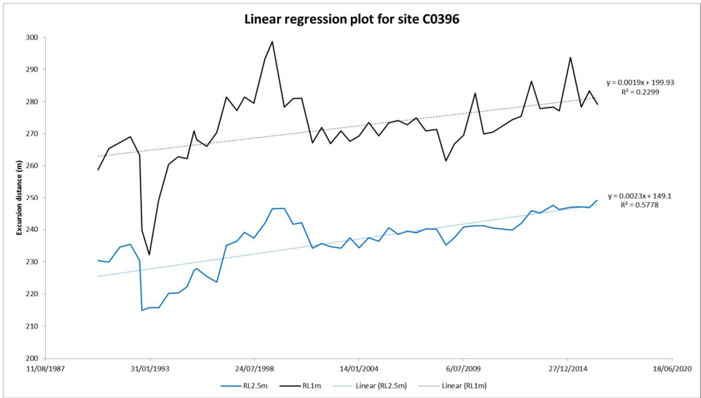
Figure B25 Beach profile surveys (top panel) and linear regression plots for RL 2.5 m and RL 1 m contours (lower panel) for profile C0396
