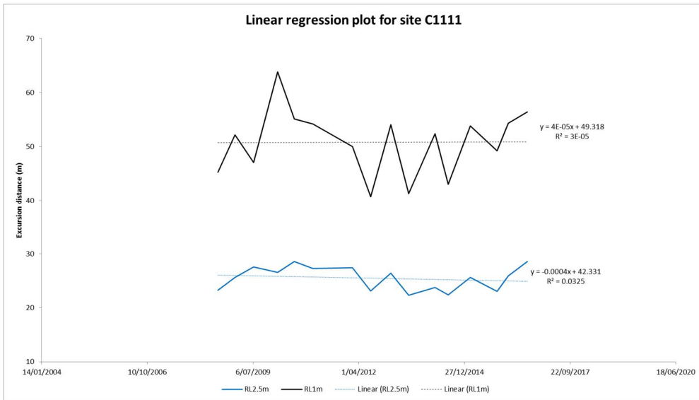
Figure B2 Beach profile surveys (top panel) and linear regression plots for RL 2.5 m and RL 1 m contours (lower panel) for profile C1111
