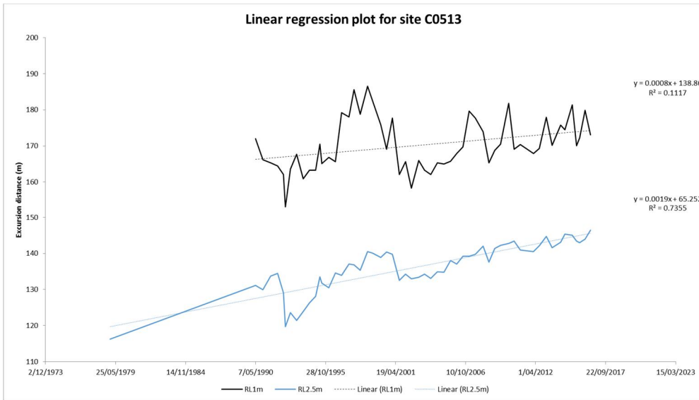
Figure B22 Beach profile surveys (top panel) and linear regression plots for RL 2.5 m and RL 1 m contours (lower panel) for profile C0513
