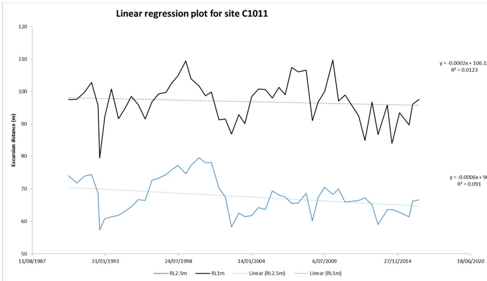
Figure B7 Beach profile surveys (top panel) and linear regression plots for RL 2.5 m and RL 1 m contours (lower panel) for profile C1011
