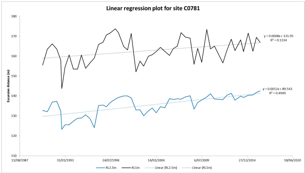
Figure B16 Beach profile surveys (top panel) and linear regression plots for RL 2.5 m and RL 1 m contours (lower panel) for profile C0781
