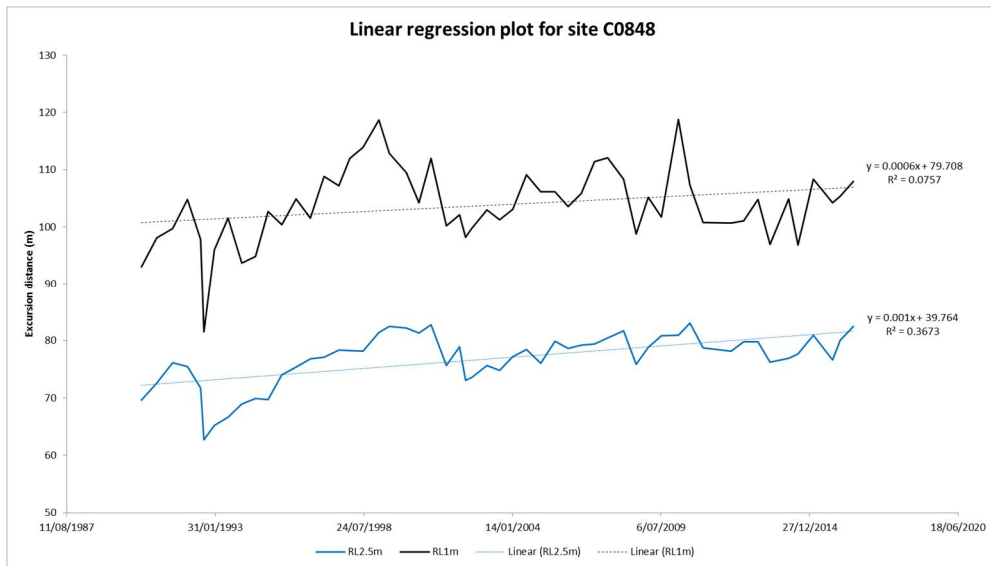
Figure B14 Beach profile surveys (top panel) and linear regression plots for RL 2.5 m and RL 1 m contours (lower panel) for profile C0848
