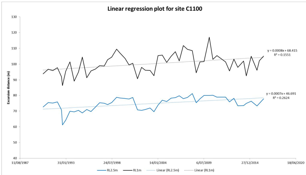
Figure B3 Beach profile surveys (top panel) and linear regression plots for RL 2.5 m and RL 1 m contours (lower panel) for profile C1100
