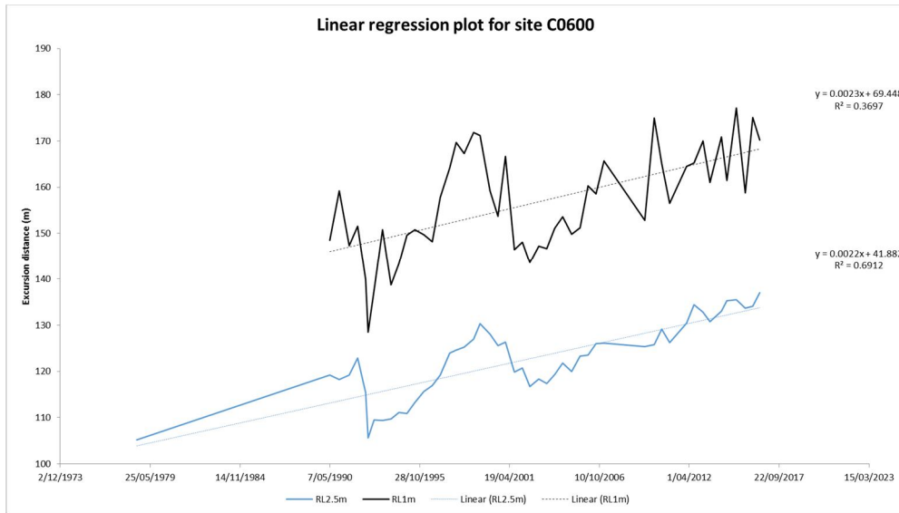
Figure B20 Beach profile surveys (top panel) and linear regression plots for RL 2.5 m and RL 1 m contours (lower panel) for profile C0600
