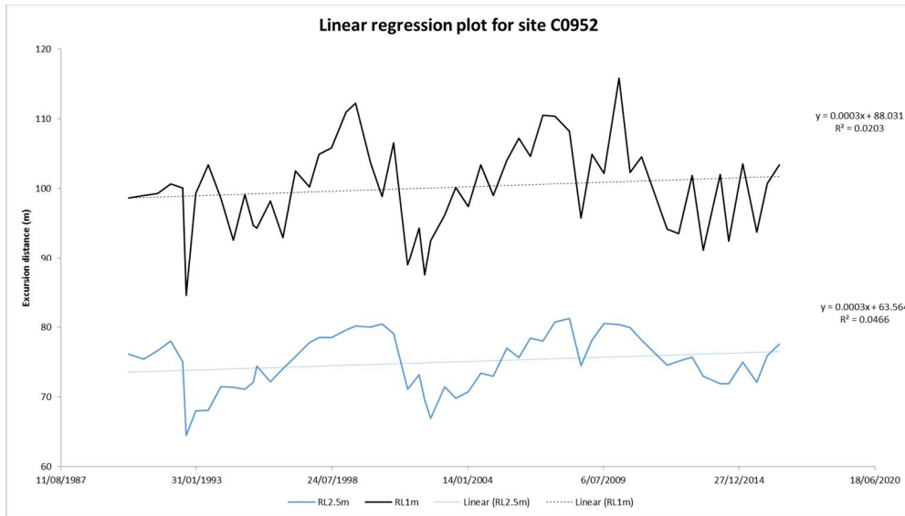
Figure B8 Beach profile surveys (top panel) and linear regression plots for RL 2.5 m and RL 1 m contours (lower panel) for profile C0952
