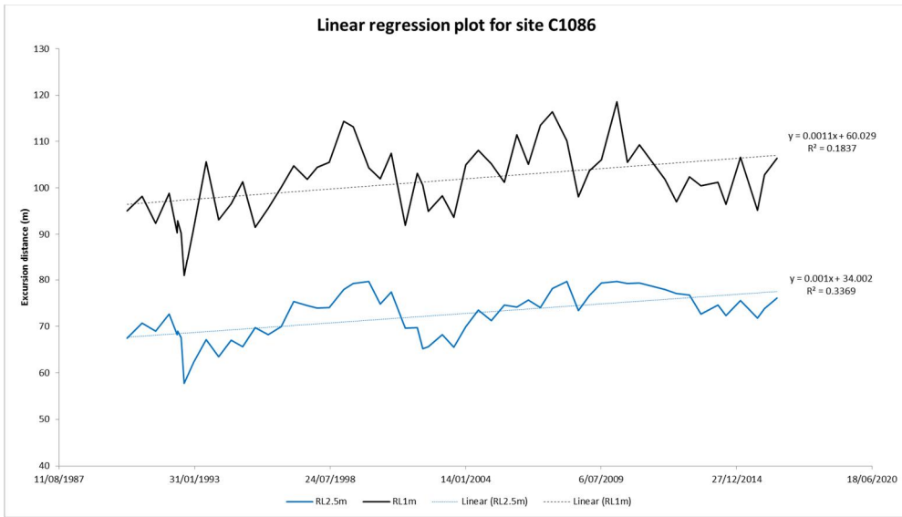
Figure B4 Beach profile surveys (top panel) and linear regression plots for RL 2.5 m and RL 1 m contours (lower panel) for profile C1086
